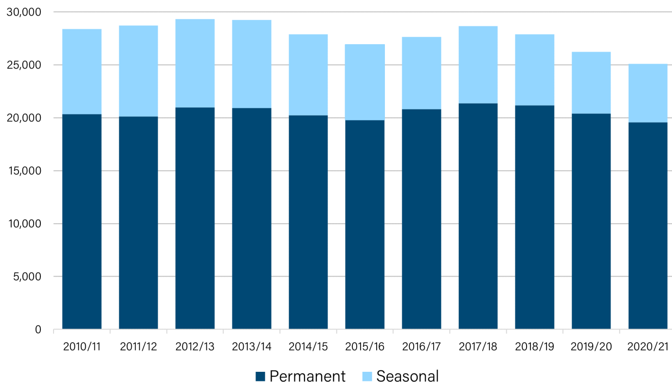
Figure 10: Sugar industry employment during the beet processing campaign
